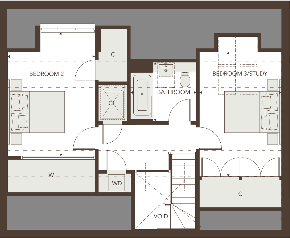
SECOND FLOOR
